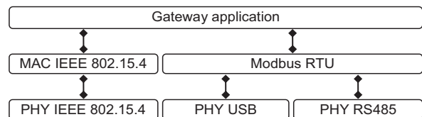
Figure 4. Gateway layers.
