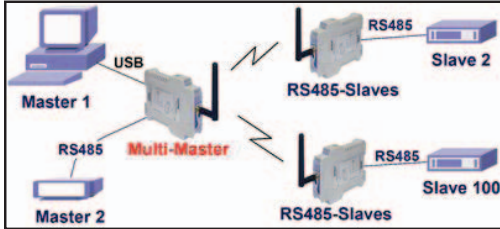
Figure 8. Operation Mode Multi-Master.
