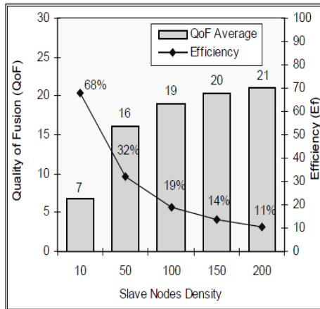
Figure 4. IEEE 802.15.4 simulated behaviour.
