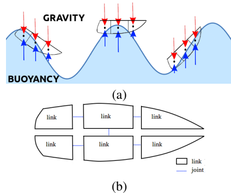
Figure 2: The black dots represent the center of buoyancy, while red and blue arrows represent, respectively, the gravity and buoyancy force vectors. In (a), the resulting buoyancy effect of the boat when represented by a set of links and joints (b). Note that the gravity and buoyancy forces are applied to each of the links' center of buoyancy.
