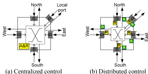
Fig. 2. Router architectures (B: input buffer, A: arbitration, R: routing logic).
