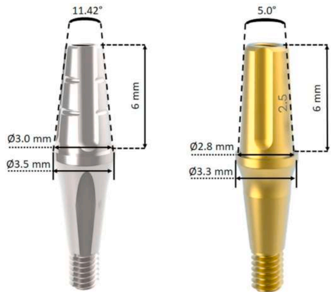
Fig. 1. Dimensional characteristics of the Smart abutment (left) and Ideale abutment (right).
