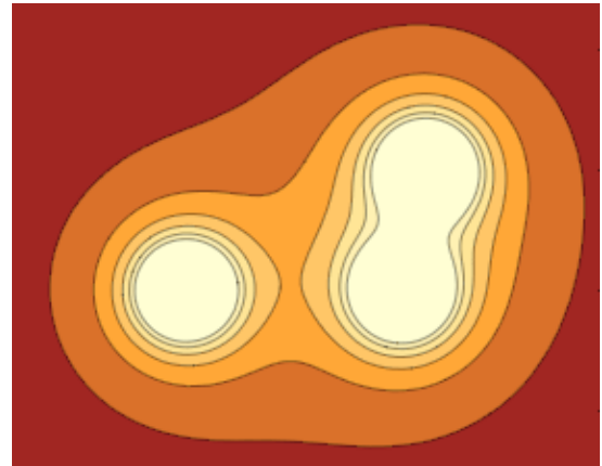
Fig. 2. Isolines representing a blobby model for several threshold values.
