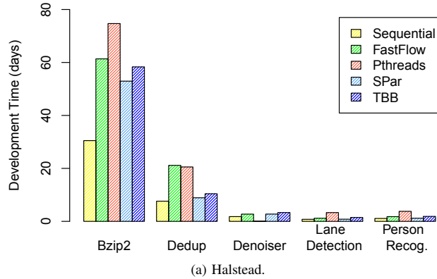
Fig. 1: Results of development time estimated.
