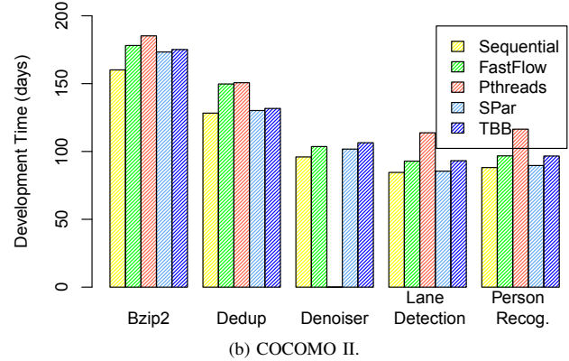
Fig. 1: Results of development time estimated.
