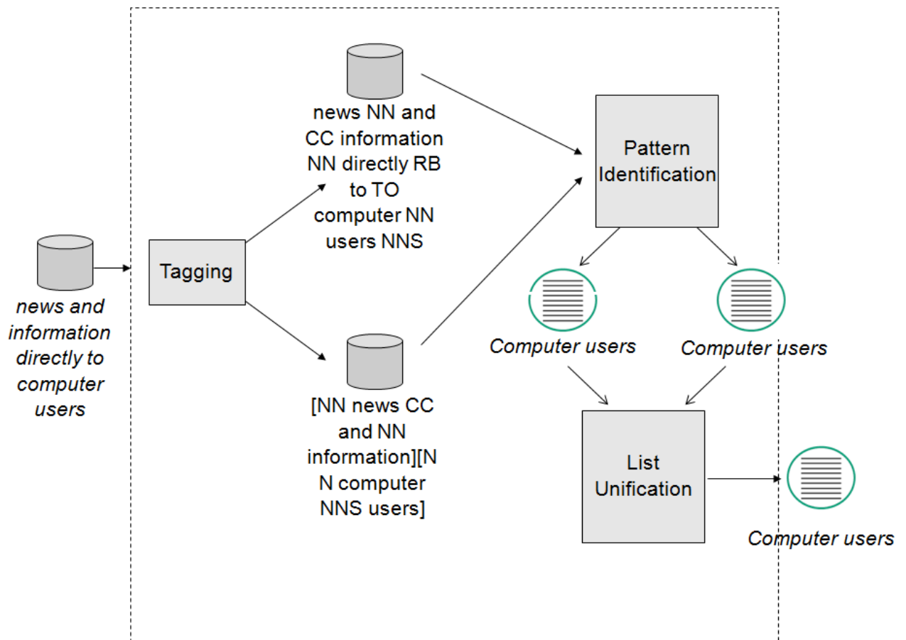
Figure 16. NCs and ANs Extraction for the sentence news and information directly to computer users .
