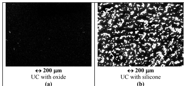
Figure 1. SEM pictures at a magnification of 95 commercial UCs increases attached in spin-on oxide (a) and silicone gel (b) [18].
