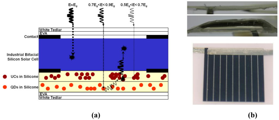
Fig. 4. (a) Encapsulation scheme: industrial BSSC laminated to UC and QDs in silicone. * represents the generation of an electron-hole pair and \blacktriangle the UC phenomena. (b) Pictures of the developed encapsulation: cross section with silicone+UC+QDs (above) and frontal view (below)
