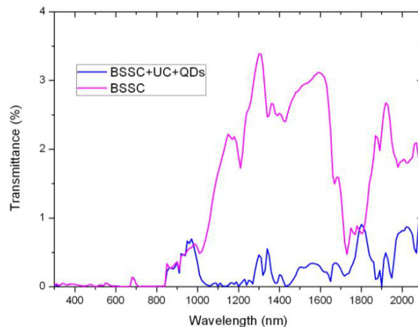
Figure 6. Transmittance of an encapsulated BSSC with and without UC and QDs embedded in the silicone.
