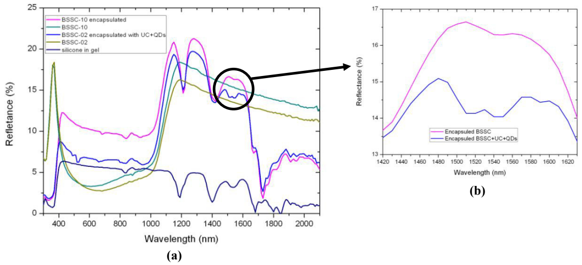
Figure 5. (a) Reflectance of the encapsulated BSSC with and without UC and QDs embedded in the silicone and (b) zoom of the reflectance in the range 1420 nm-1640 nm ( {}^4I_{13/2} ( {}^4I_{15/2} ) \text{Er}^{3+} ion transitions).
