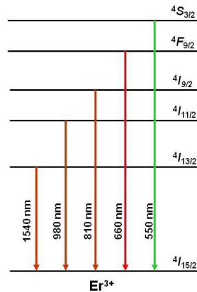
Fig. 3. Emissions of the Er^{3+} doped materials under excitation around 1500 nm.
