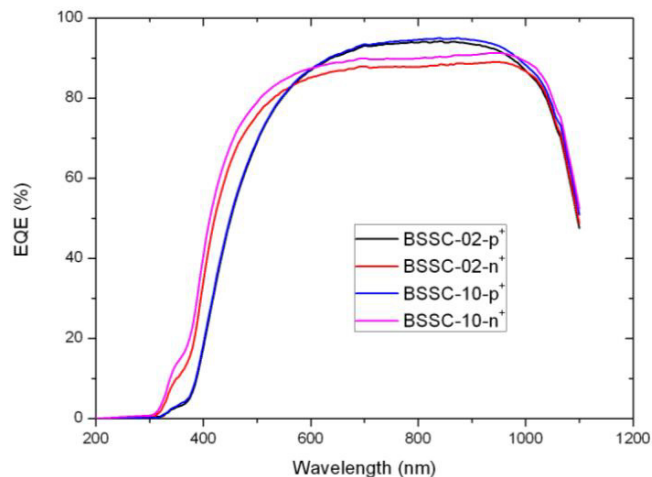
Fig. 2. External quantum efficiency of two BSSC developed in n-type Cz substrates for both illumination modes.
