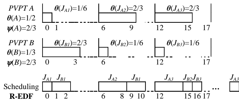
Figure 3: Reservation in R-EDF with two PVPT tasks
